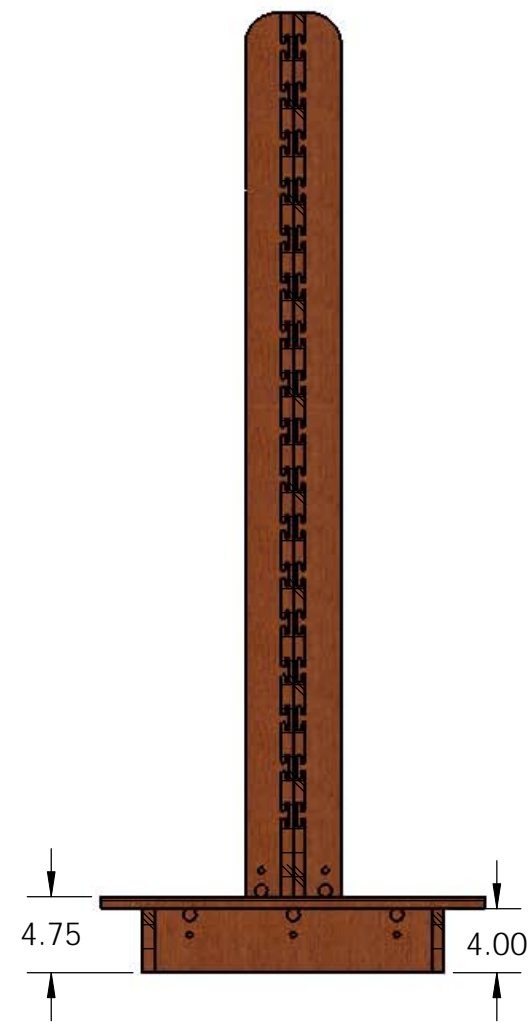
SECTION B-B
